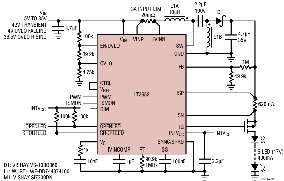
SEPIC LED Driver with Input Current Limit
