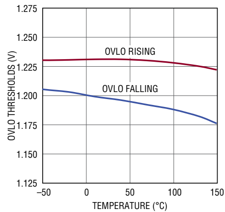
OVLO Thresholds vs Temperature
