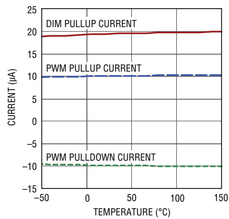
PWM Generator Currents vs Temperature
