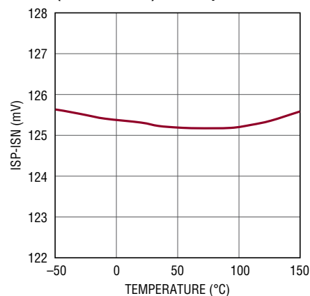
ISP/ISN Mid-Scale Threshold (CTRL = 0.7V) vs Temperature
