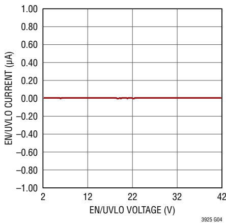
EN/UVLO Bias Current above Threshold
