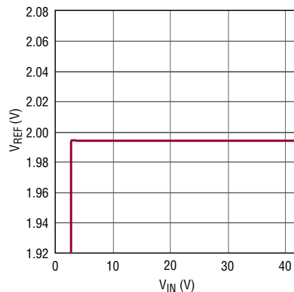
Reference Voltage vs Input Voltage
