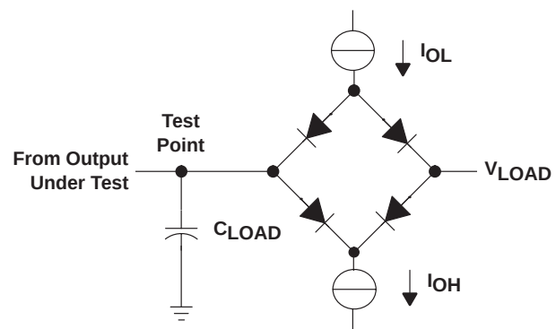
LOAD CIRCUIT
