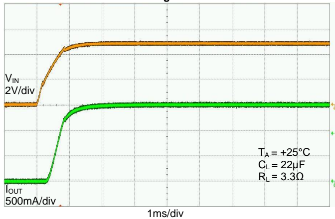
UVLO Increasing With Full Load
