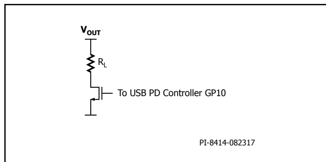
Figure 12. Active Pre-Load Circuit.
