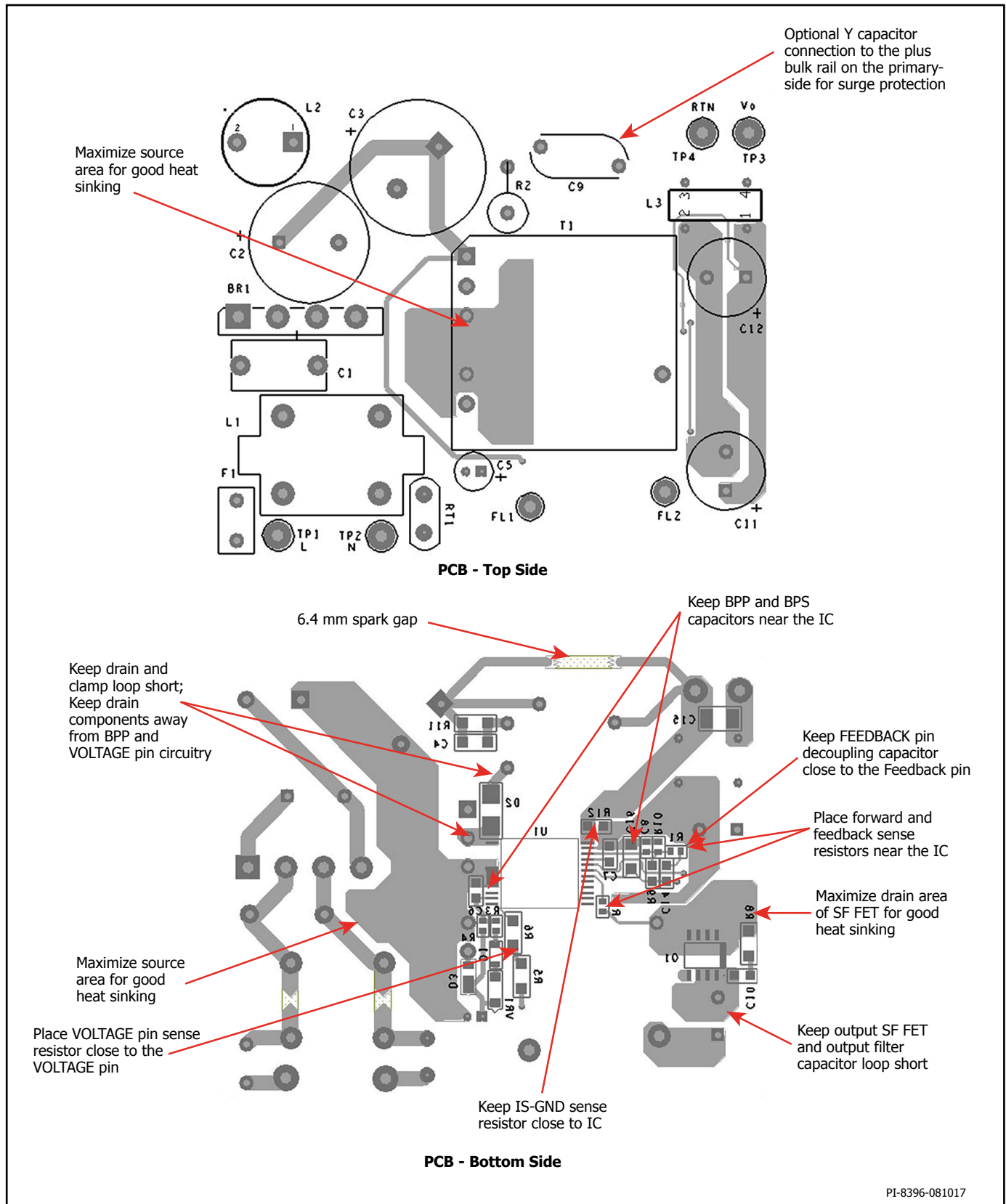
Figure 19. PCB.
