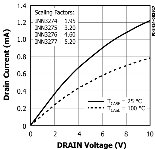
Figure 29. Output Characteristics.
