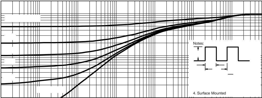
Safe Operating Area
