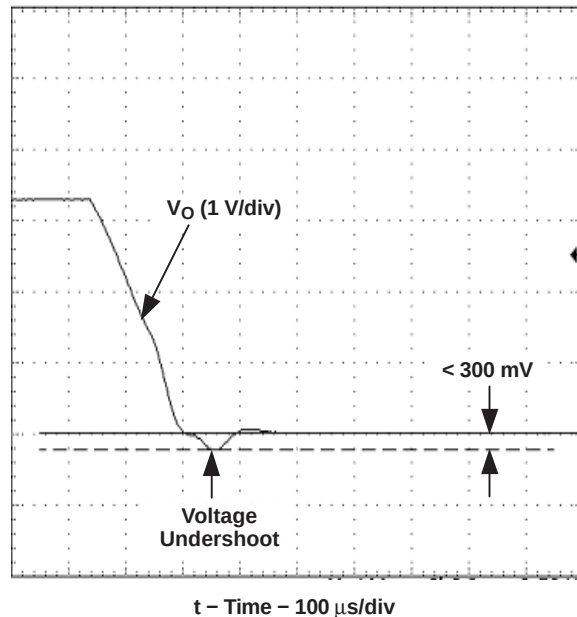
Figure 15. Power Down
