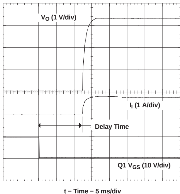
Figure 14. Power Up
