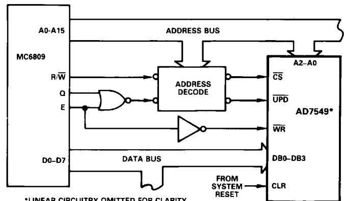
Figure 8. AD7549-MC6809 Interface
