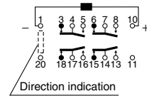
1-coil latching
