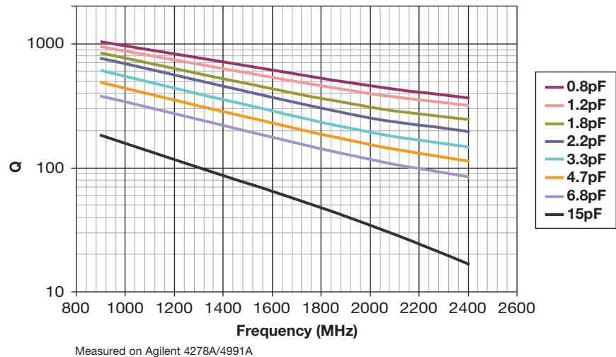
Accu-P® 1210 Typical Q vs Frequency
