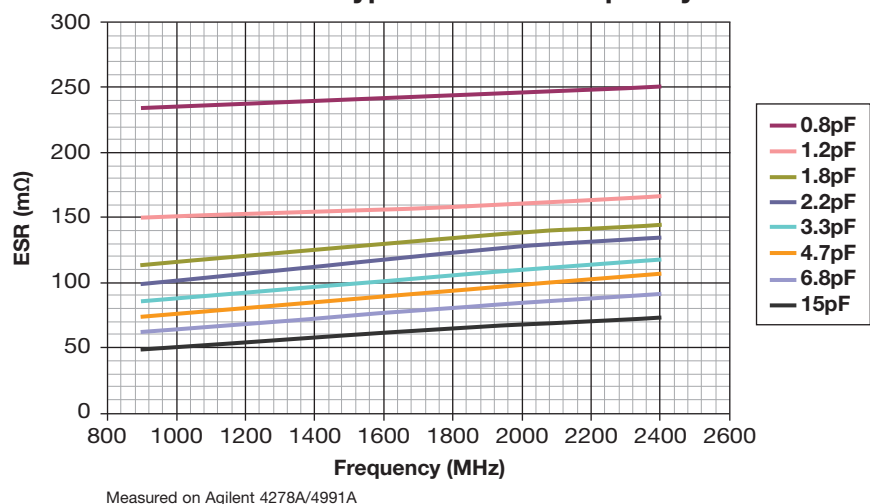
Accu-P® 1210 Typical ESR vs Frequency
