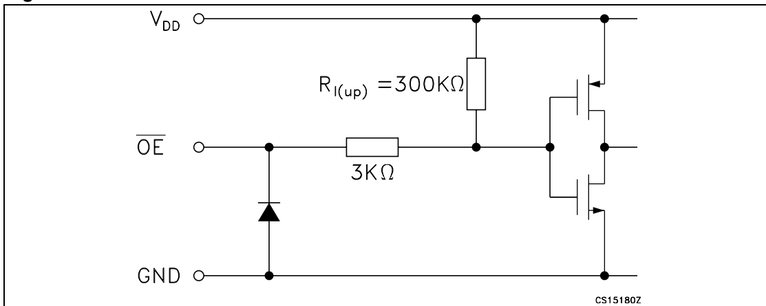
Figure 2. \overline{\text{OE}} terminal
