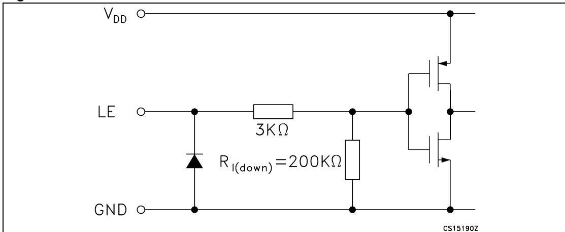
Figure 3. LE terminal
