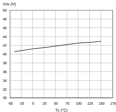
Figure 19. Overvoltage shutdown
