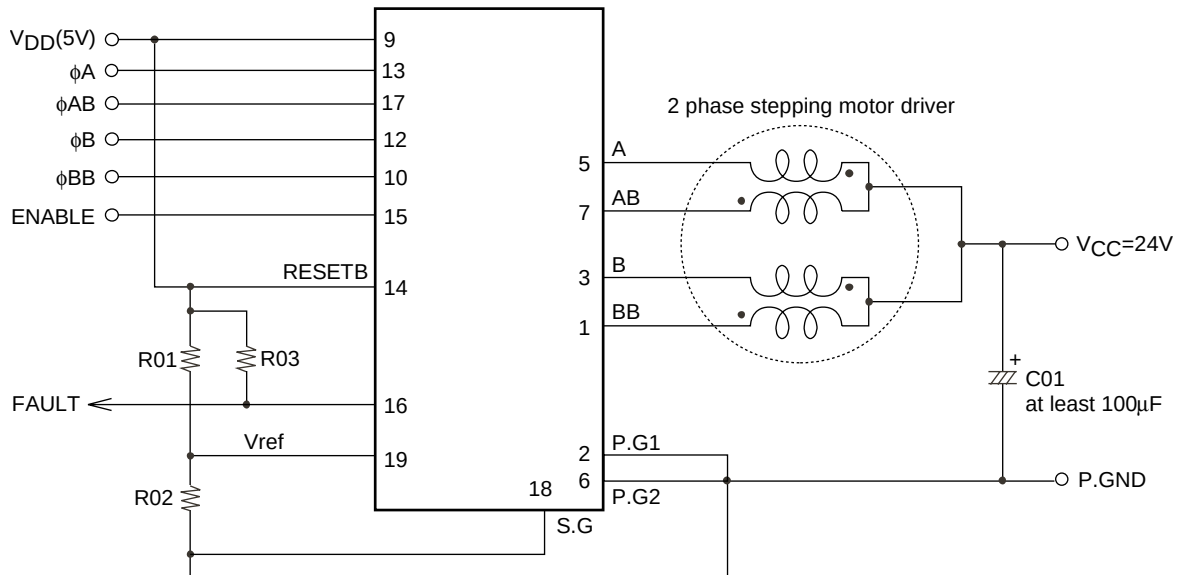
STK672-732A-E
