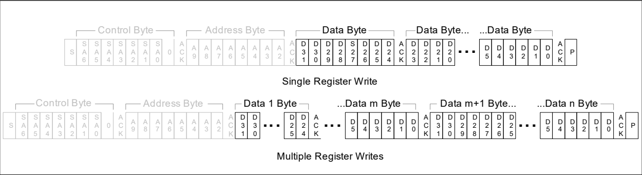
FIGURE 11-4: I 2 C TARGET WRITES
