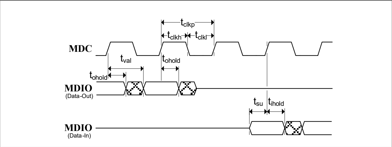
FIGURE 14-1: SMI TIMING
