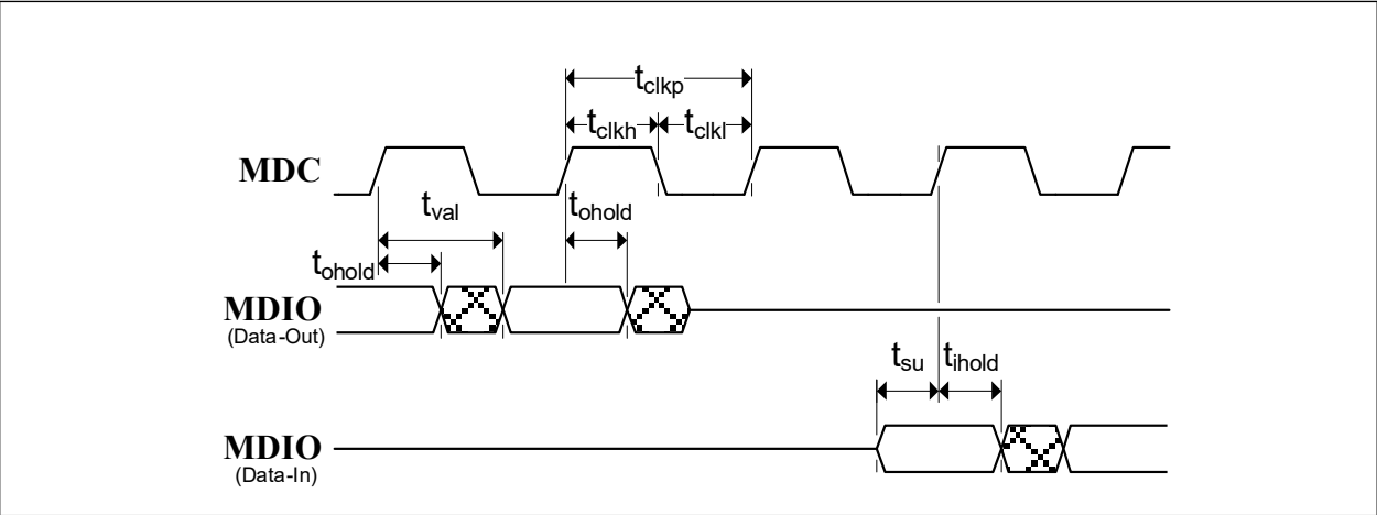
FIGURE 14-2: PMI TIMING
