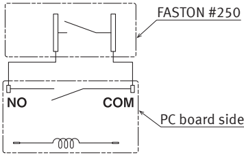
Schematic (Bottom view)
