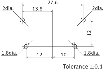
Schematic (Bottom view)
