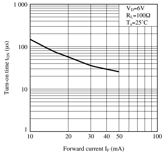
Fig.8-b Turn-on Time vs. Forward Current (S201D01)
