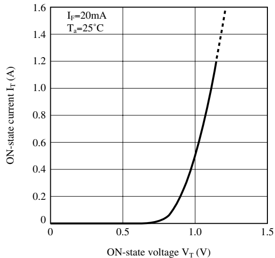
Fig.7-b ON-state Current vs. ON-state Voltage (S201D01)
