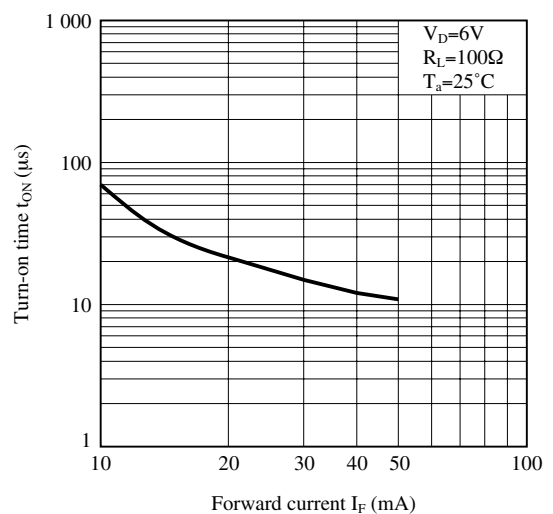
Fig.8-a Turn-on Time vs. Forward Current (S101D01)
