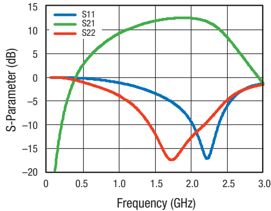
Figure 91. S-Parameter vs Frequency, Tuned for 2140 MHz
