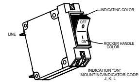
MARKING DETAIL "A"
