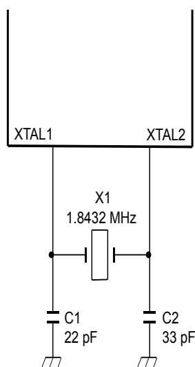
Figure 8. Crystal oscillator circuit reference
