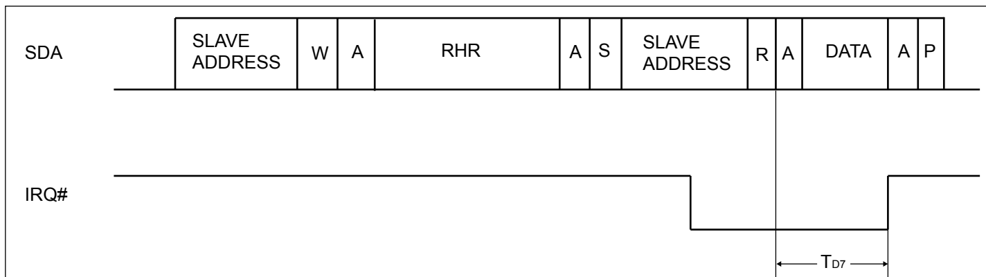
Figure 7. Receive Interrupt Clear
