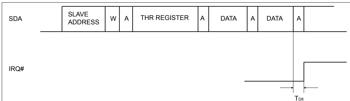
Figure 8. Transmit Interrupt Clear
