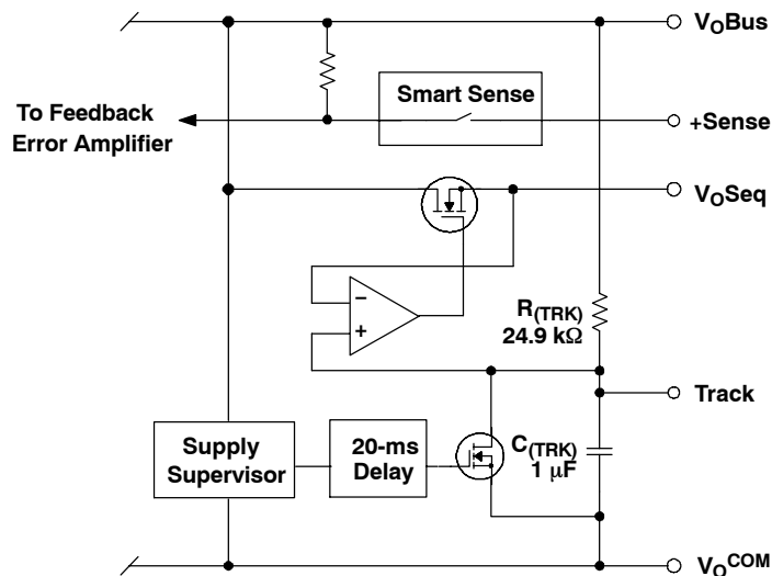
Figure 8. Block Diagram of Auto-Track Features
