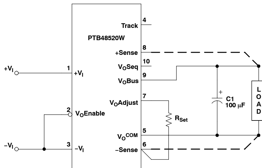
Figure 11. Stand-Alone Configuration
