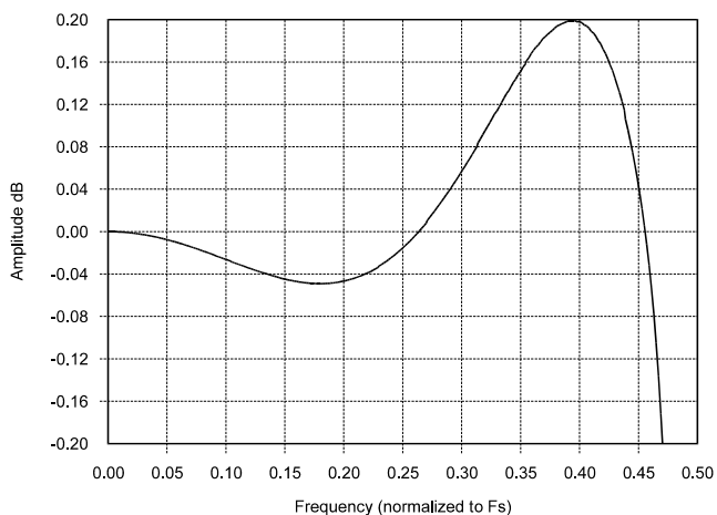
Figure 22. Passband Ripple
