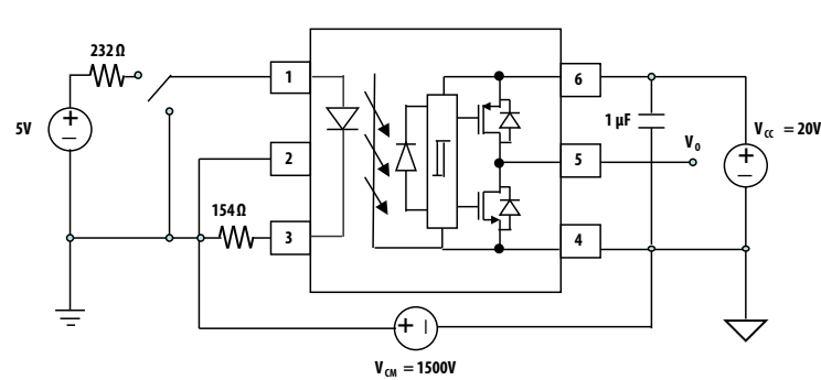
Figure 21: CMR Test Circuit with Split Resistors Network
