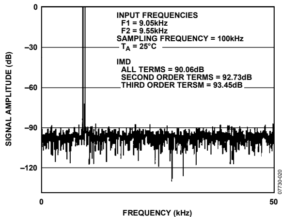
Figure 20. IMD Plot
