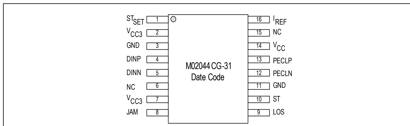
Figure 2-1. M02044CG-31 Pinout
