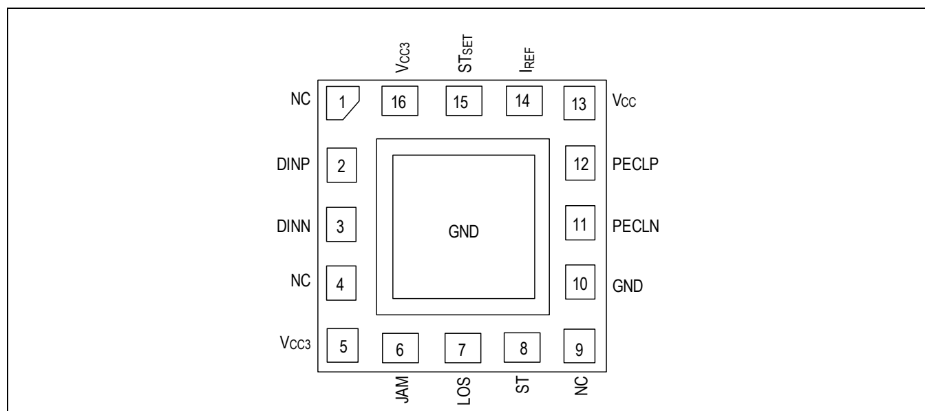
Figure 2-2. M02044CG-61 Pinout
