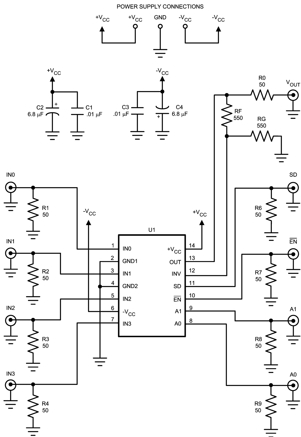
FIGURE 1. Board Schematic
