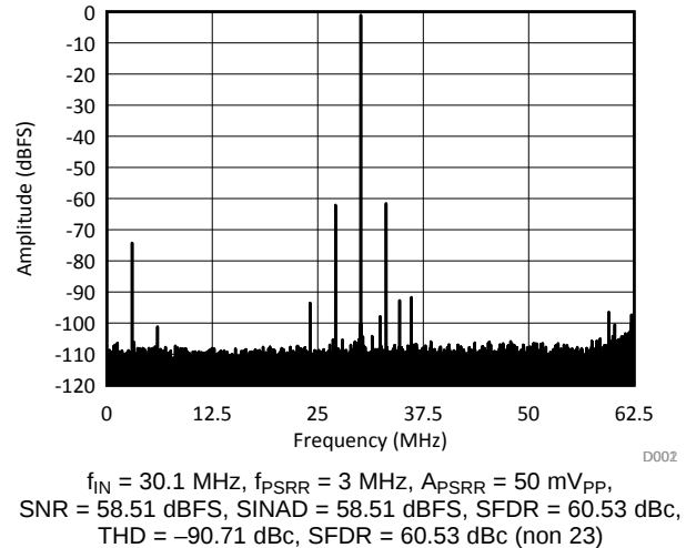
Figure 126. Power-Supply Rejection Ratio Spectrum
