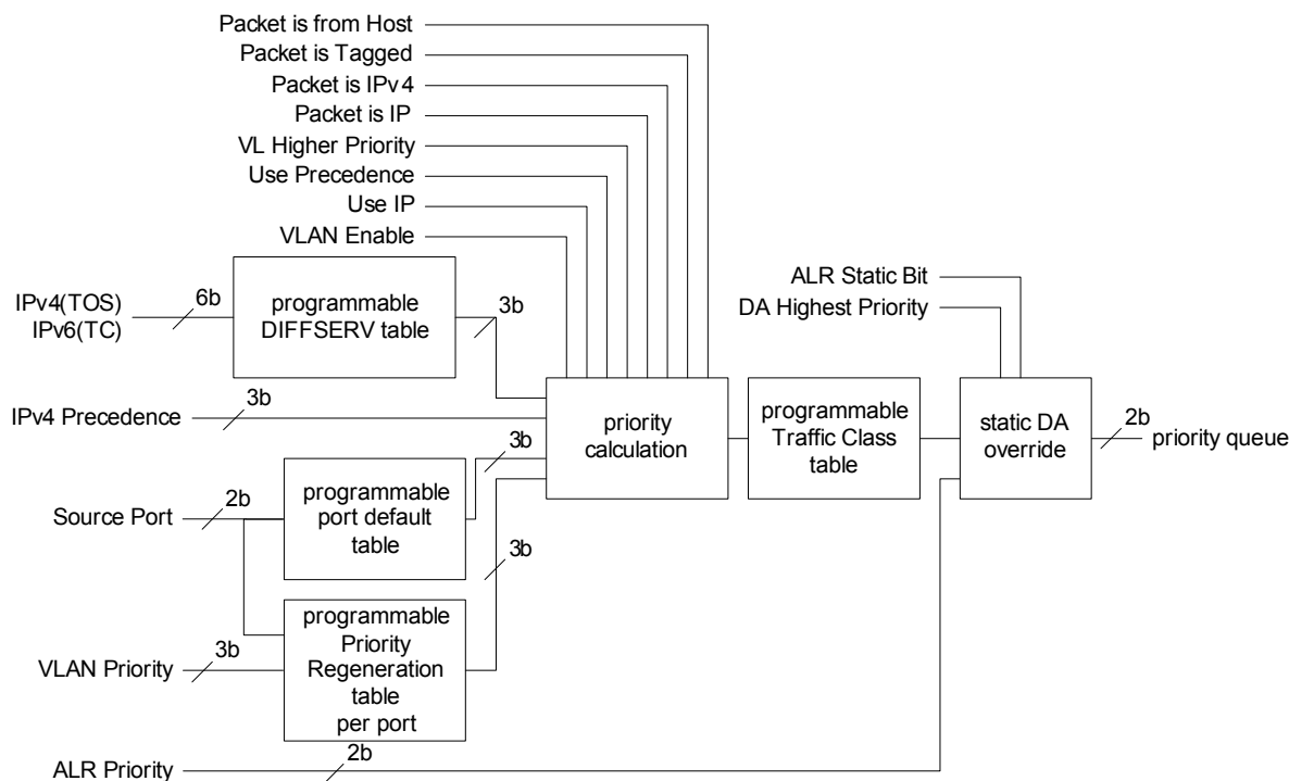
Figure 6.4 Switch Engine Transmit Queue Selection
