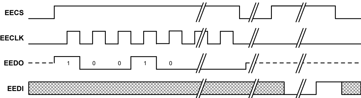
Figure 10.8 EEPROM ERAL Cycle
