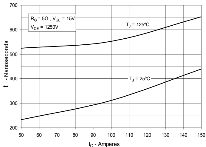
Fig. 13. Resistive Turn-on Rise Time vs. Collector Current
