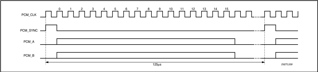
Figure 20. Linear mode
