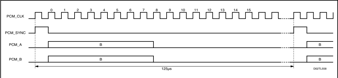
Figure 19. PCM (A-law, \mu -law) standard mode
