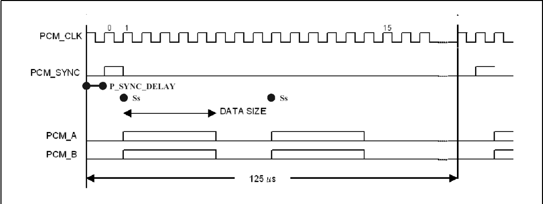
Figure 21. Multislot operation
