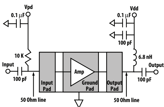
Figure 14. Example demonstration circuit of VMMK-3803 for broadband operation (3GHz to 11GHz).
