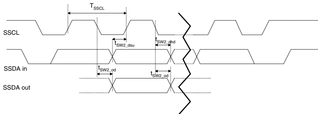
Figure 7-11 2-wire slave timing diagram
