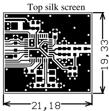
Figure 18-3 nRF24Z1 ATX PCB layout
