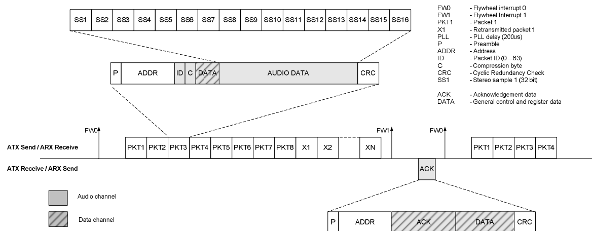
Figure 4-4 nRF24Z1 data frame and packet organization
