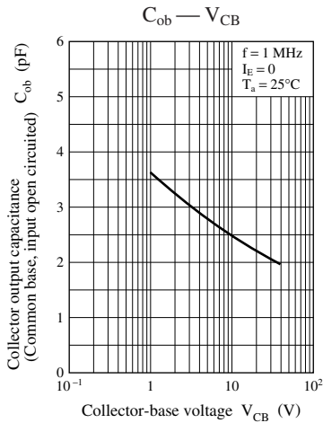
Characteristics charts of UNR521K
