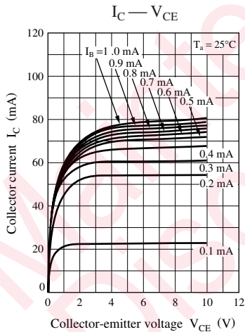
Characteristics charts of UNR5217
