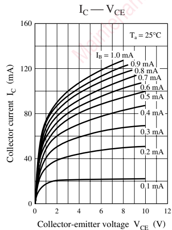
Characteristics charts of UNR5216
