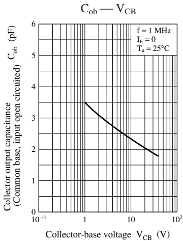
Characteristics charts of UNR5217
