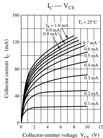
Characteristics charts of UNR5215
