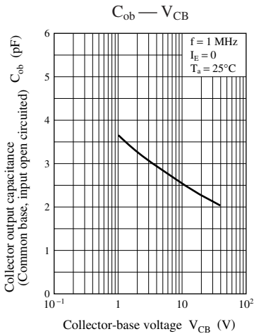
Characteristics charts of UNR521D
