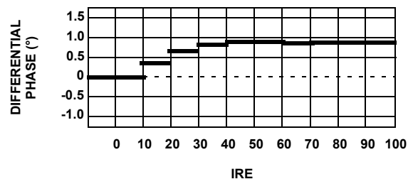
FIGURE 36. DIFFERENTIAL PHASE
