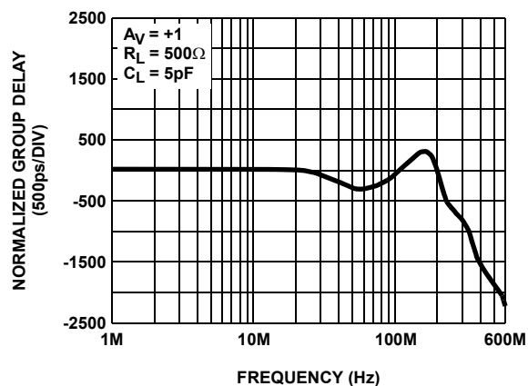
FIGURE 22. GROUP DELAY
