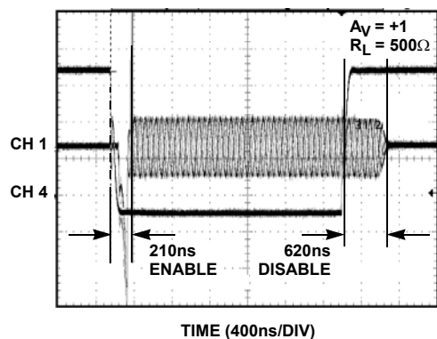
FIGURE 33. EL5150 ENABLE/DISABLE
