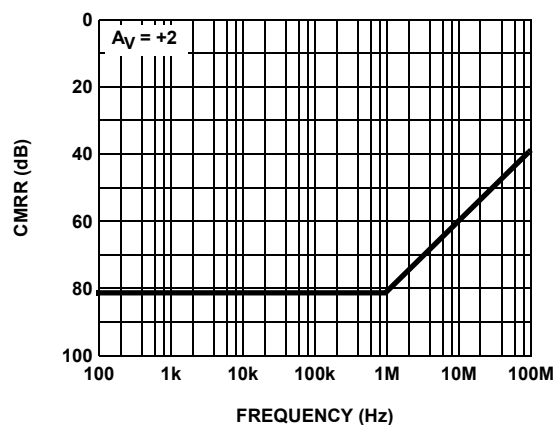
FIGURE 21. CMRR
