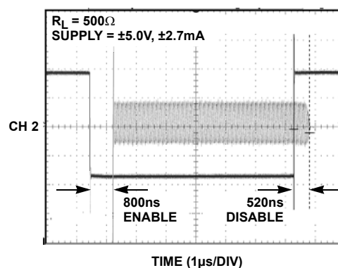
FIGURE 34. EL5250 ENABLE/DISABLE
