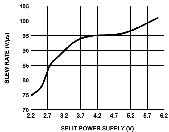
FIGURE 26. SLEW RATE vs POWER SUPPLY
