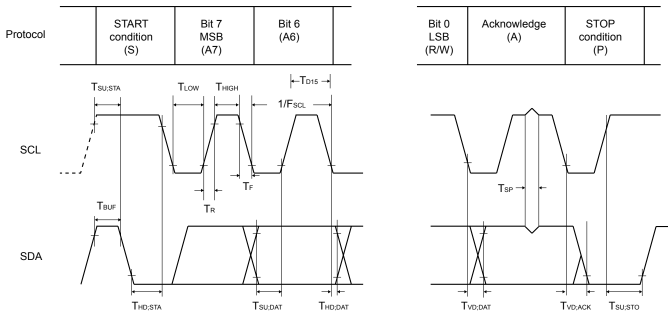
Figure 2. I²C-Bus Timing Diagram
