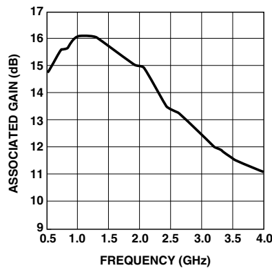
Figure 15. Associated Gain vs. Frequency at V_{dd} = 5V .
