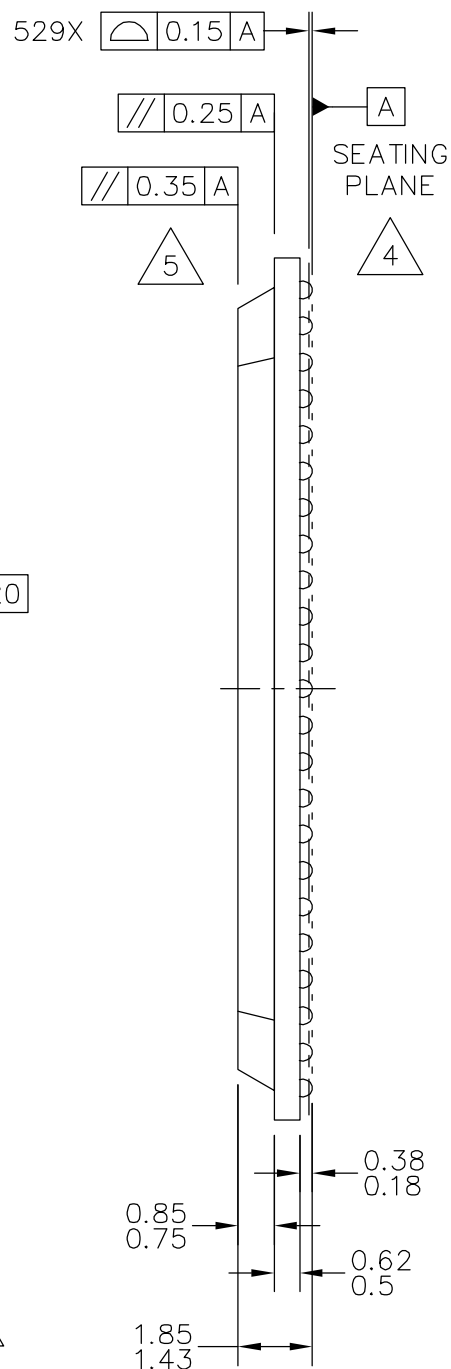
SIDE VIEW
