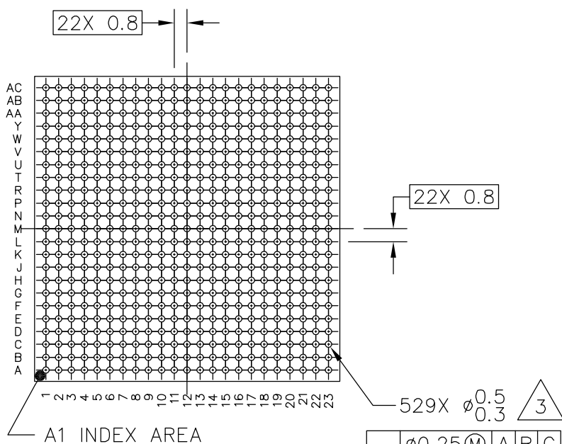
BOTTOM VIEW
