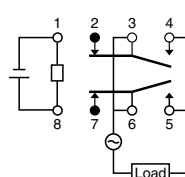
Pin layout and schematic (Bottom View)
