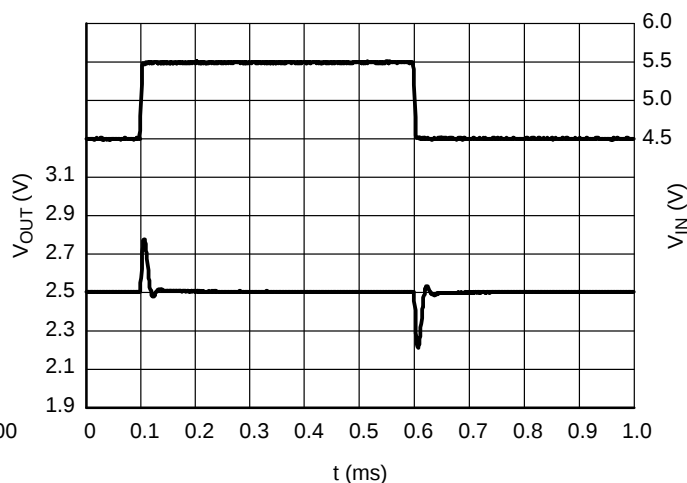
Figure 30. Line Transients, 2.5 V Version, t_R = t_F = 5 \mu\text{s} , I_{\text{OUT}} = 30 \text{ mA}
