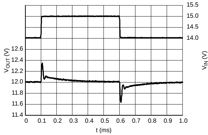
Figure 33. Line Transients, 12.0 V Version, t_R = t_F = 5 \mu s , I_{OUT} = 30 mA
