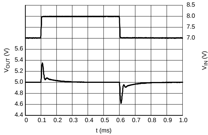
Figure 32. Line Transients, 5.0 V Version, t_R = t_F = 5 \mu s , I_{OUT} = 30 mA
