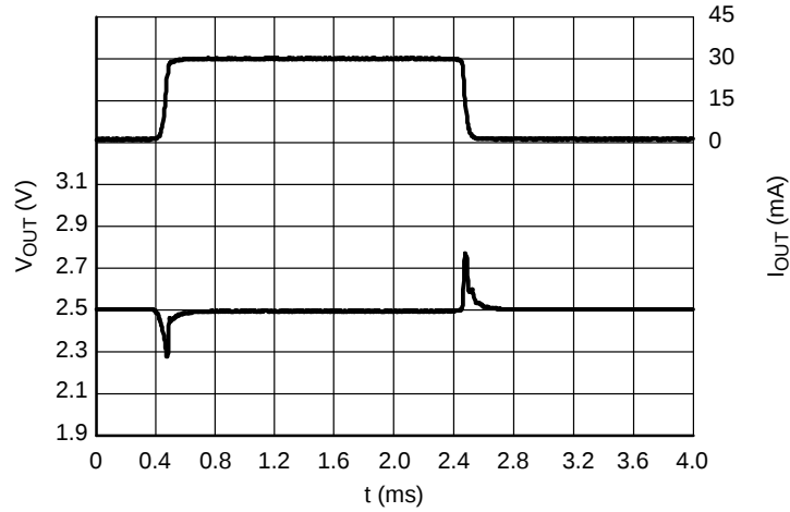
Load Transients, 2.5 V Version, I_{OUT} = 1 - 30 mA, t_R = t_F = 50 \mu s , V_{IN} = 4.5 V
