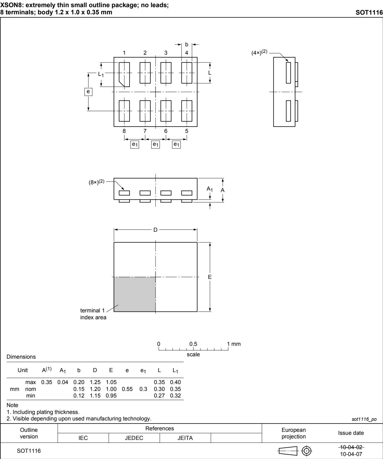
Figure 15. Package outline SOT1116 (XSON8)
