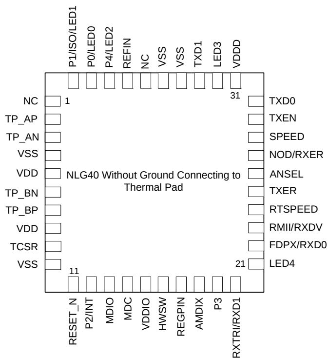
40-pin MLF
