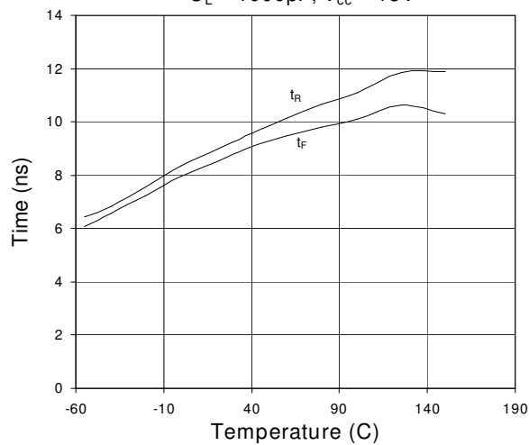
Fig. 9 Rise And Fall Times vs. Temperature C_L = 1000\text{pF} , V_{CC} = 18\text{V}
