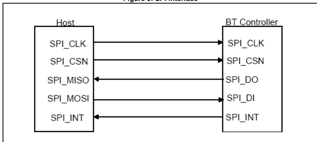
Figure 9: SPI interface
