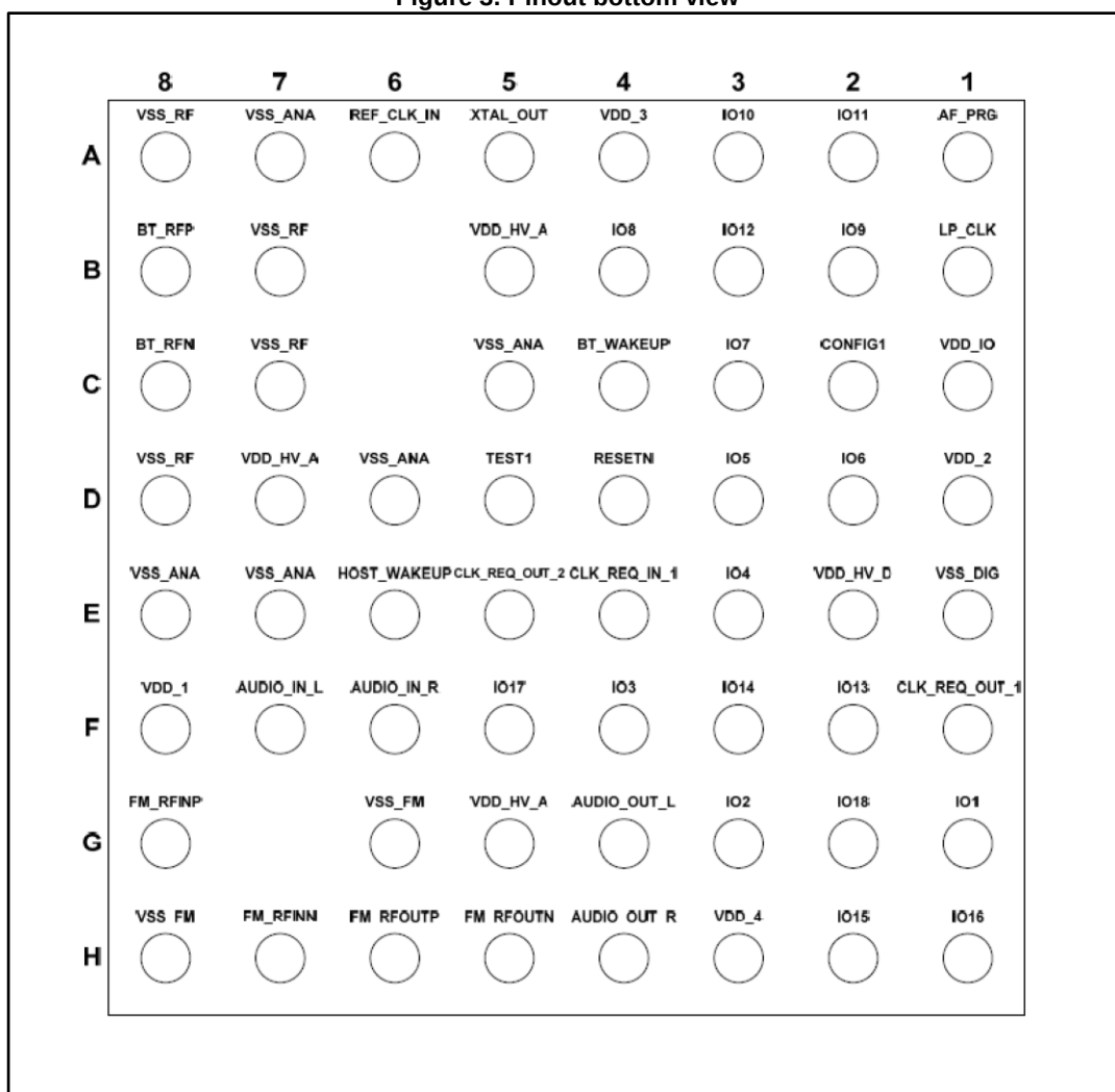
Figure 3: Pinout bottom view
