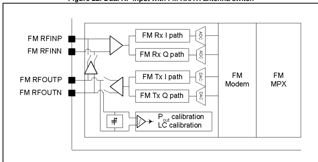
Figure 22: Dual RF input with FM RX/TX antenna switch
