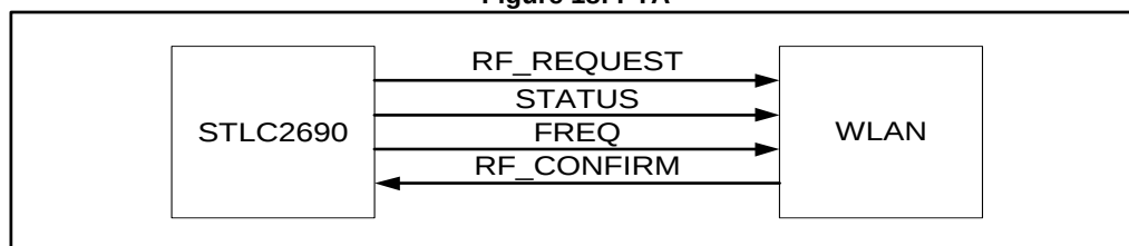
Figure 18: PTA
