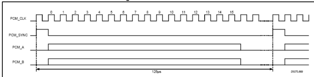
Figure 16: Multi-Slot operation
