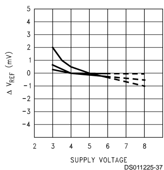
Line Regulation (3 Typical Parts)
