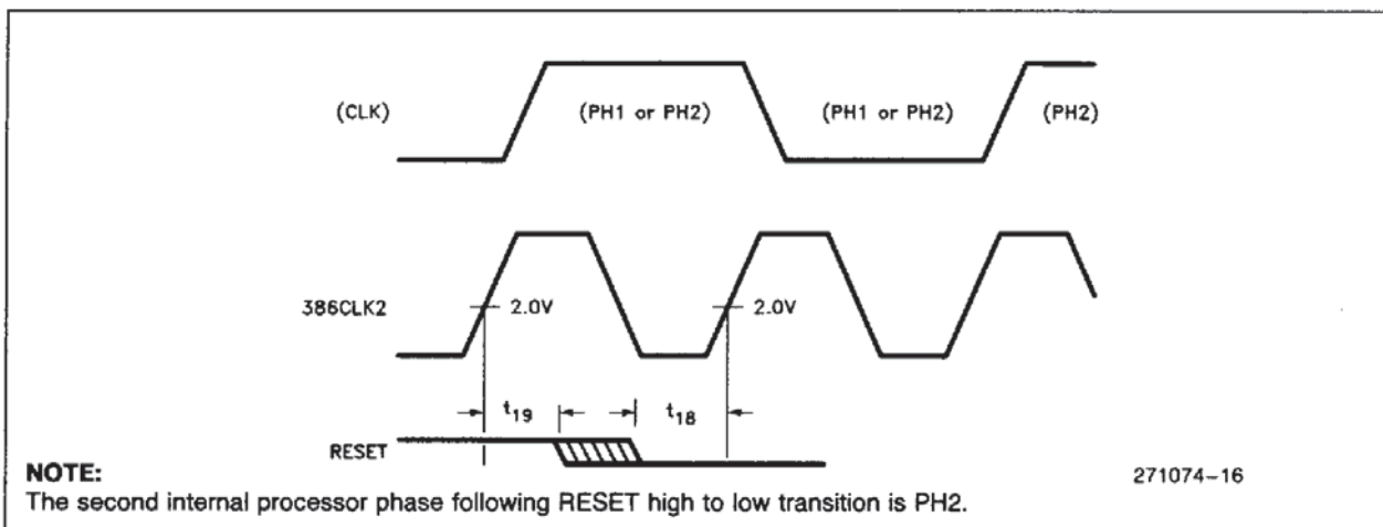
Figure 5.4. RESET Signal
