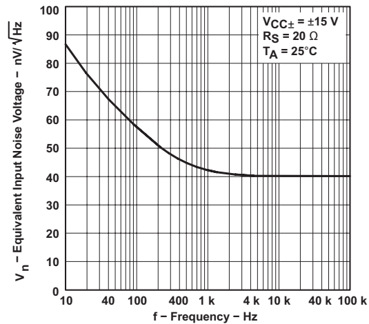
Figure 18. Equivalent Input Noise Voltage vs Frequency
