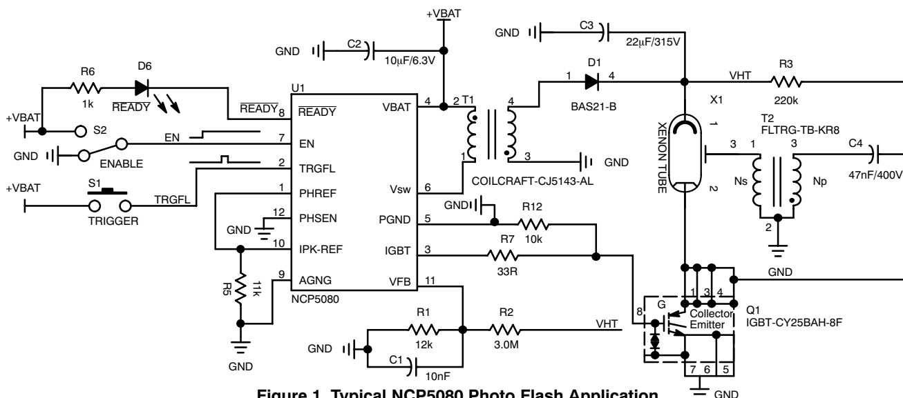
Figure 1. Typical NCP5080 Photo Flash Application
