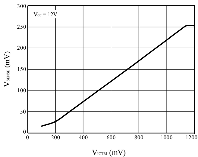
Figure 17 V_{SENSE} vs. V_{CTRL}
