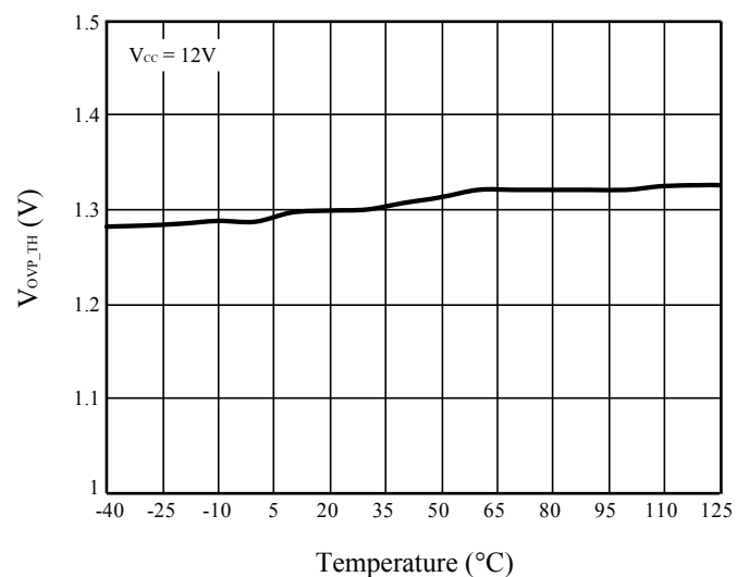
Figure 15 V_{OVP\_TH} vs. T_J
