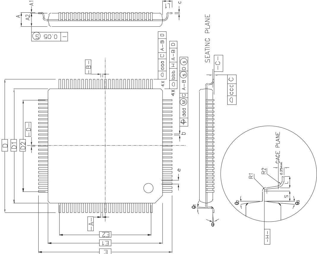
80LD 12x12x1.4 mm LQFP Package Outline Drawing
