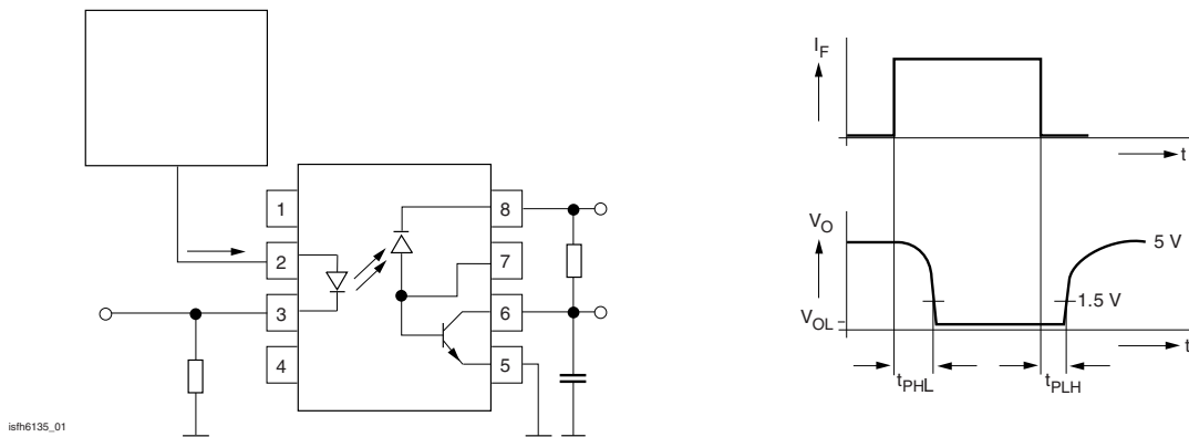
Fig. 1 - Schematics
