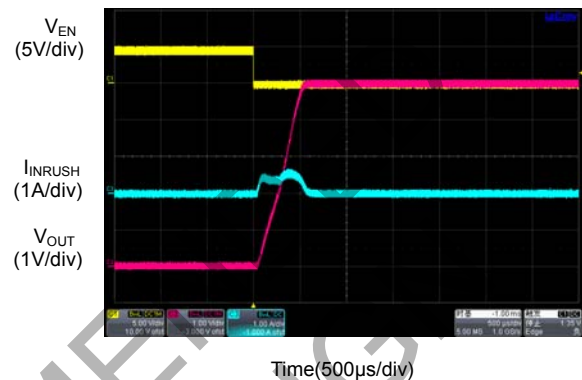
Figure 21. Output Turn ON and Rise Time ( C_{IN}=1.0\mu F, C_{OUT}=47\mu F , No Load)
