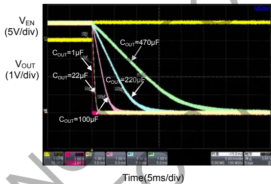
Figure 22. Output Turn OFF and Falling Time ( V_{IN}=5V, C_{IN}=1.0\mu F , No Load)
