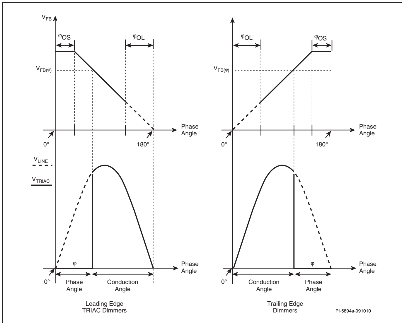
Figure 6. Feedback Voltage vs. Phase Angle Dimming Characteristics.
