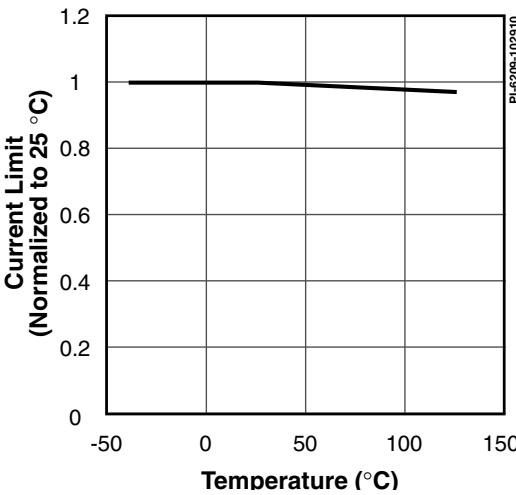
Figure 10. Standard Current Limit vs. Temperature.
