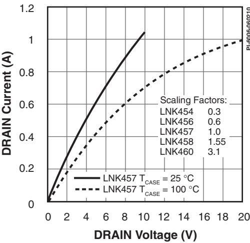
Figure 8. Drain Current vs. Drain Voltage.
