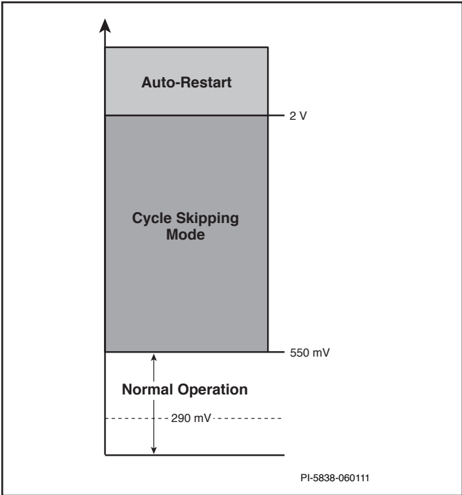
Figure 5. FEEDBACK Pin Operational Voltage Thresholds.
